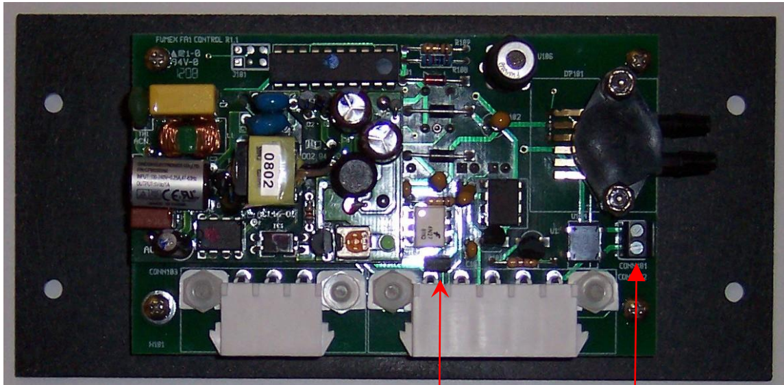
Relay activation jumper
